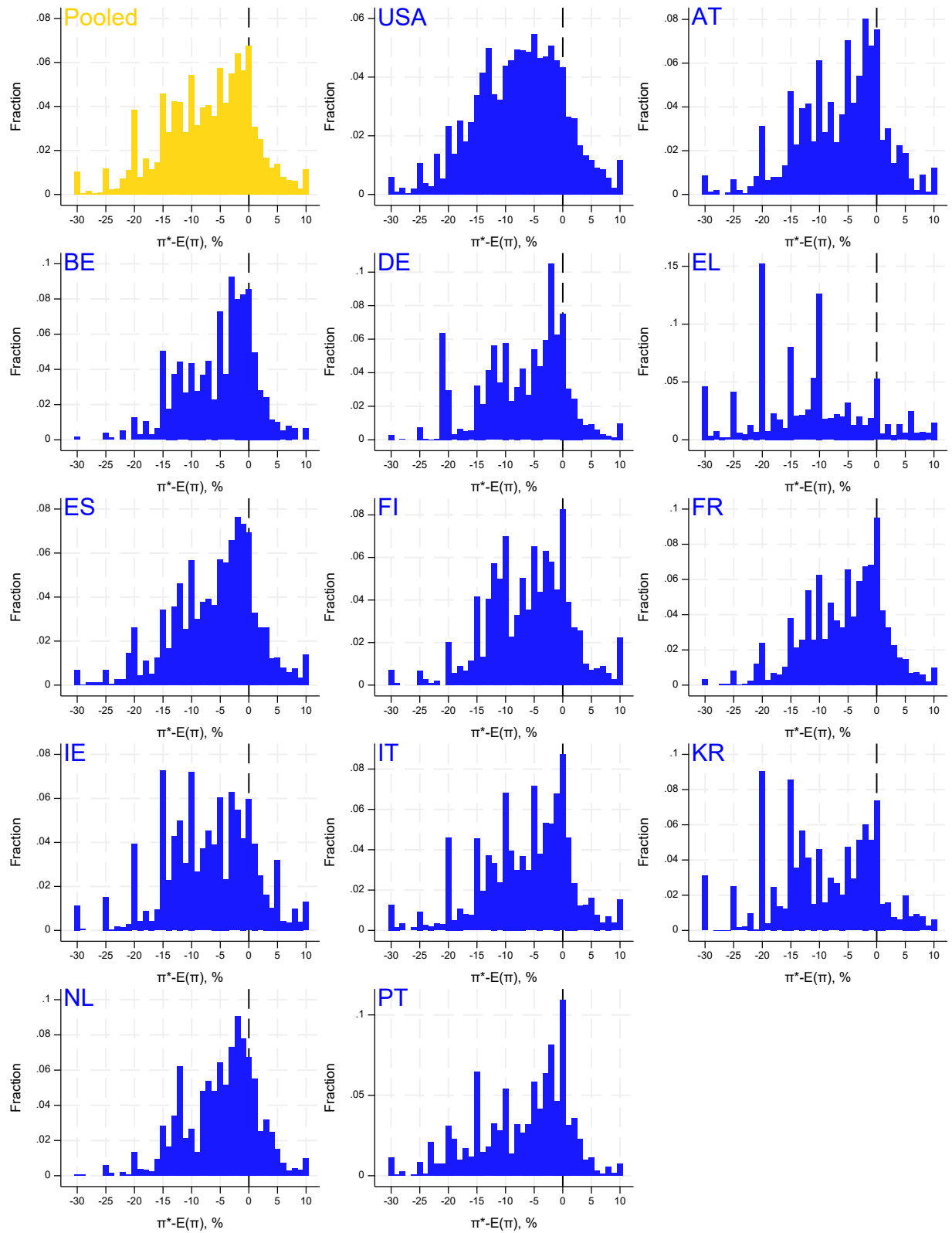
Appendix Figure 1. \pi^* - E(\pi) .
