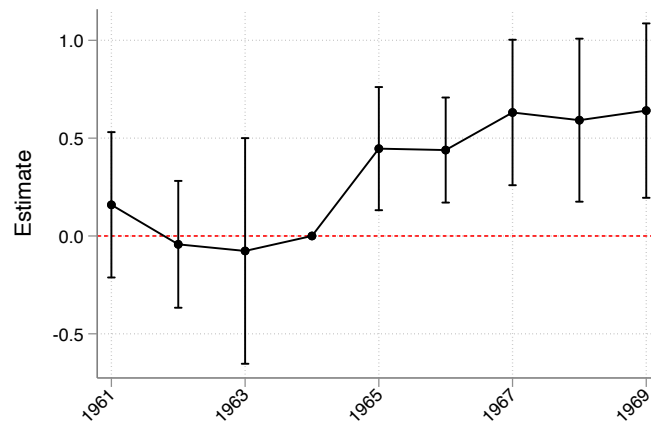
(b) Support for the first-stage parallel trends assumption
